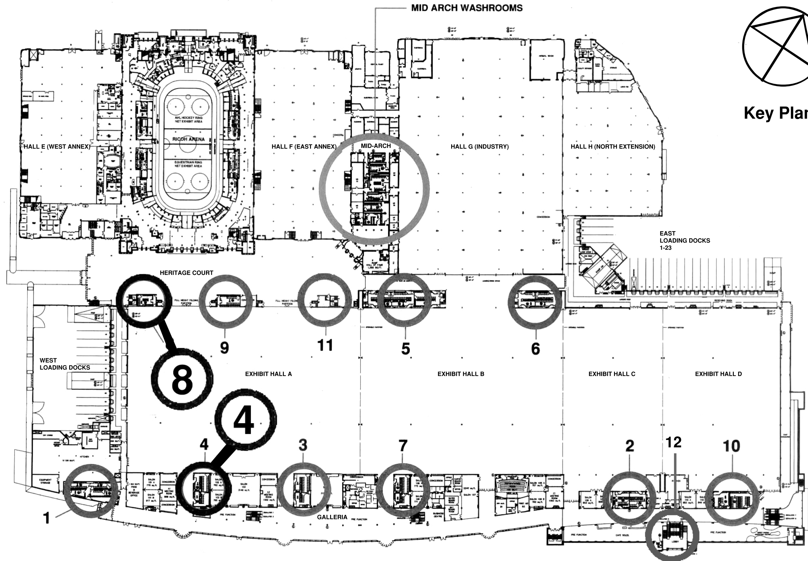
PROPOSED LOCATIONS OF WASHROOM RENOVATION DIRECT ENERGY CENTRE - MAIN FLOOR
